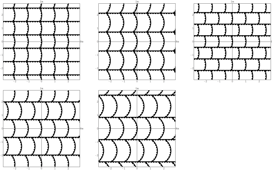
Figure 1: Tilings of \mathbb{C} given by the sets \mathbb{D}_d(p) , d \in \{1, 2, 3, 7, 11\} .
